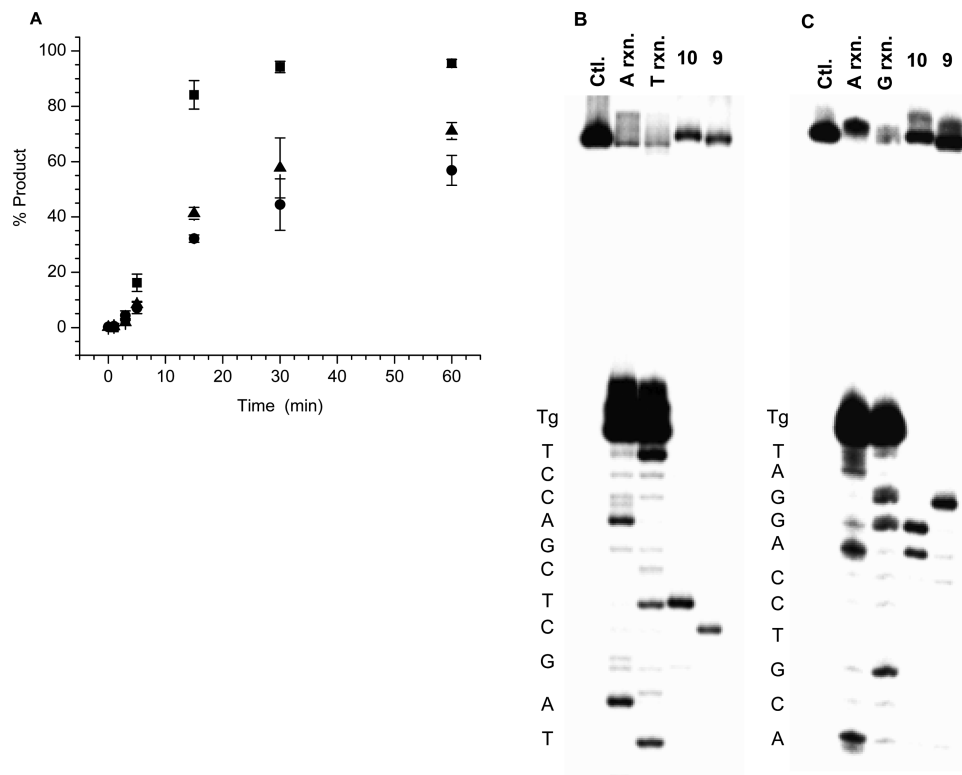
FIGURE 6: Incision of FTg tandem lesion (9), Tg (10), and fluoresceinylated standard (FI, 11) by UvrABC. (A) Incision in 5'- 32 P-labeled substrates as a function of time. FTg (9), circle; Tg (10), triangle; FI (11), square. Autoradiogram indicating the sites of incision in (B) 5'- 32 P-9 and (C) 3'- 32 P-9. Sequencing reactions selective for T (T rxn) and A (A rxn).
