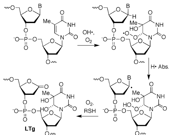
Scheme 1: Formation of the 5'-LTg Tandem Lesion from a Nucleobase Radical
