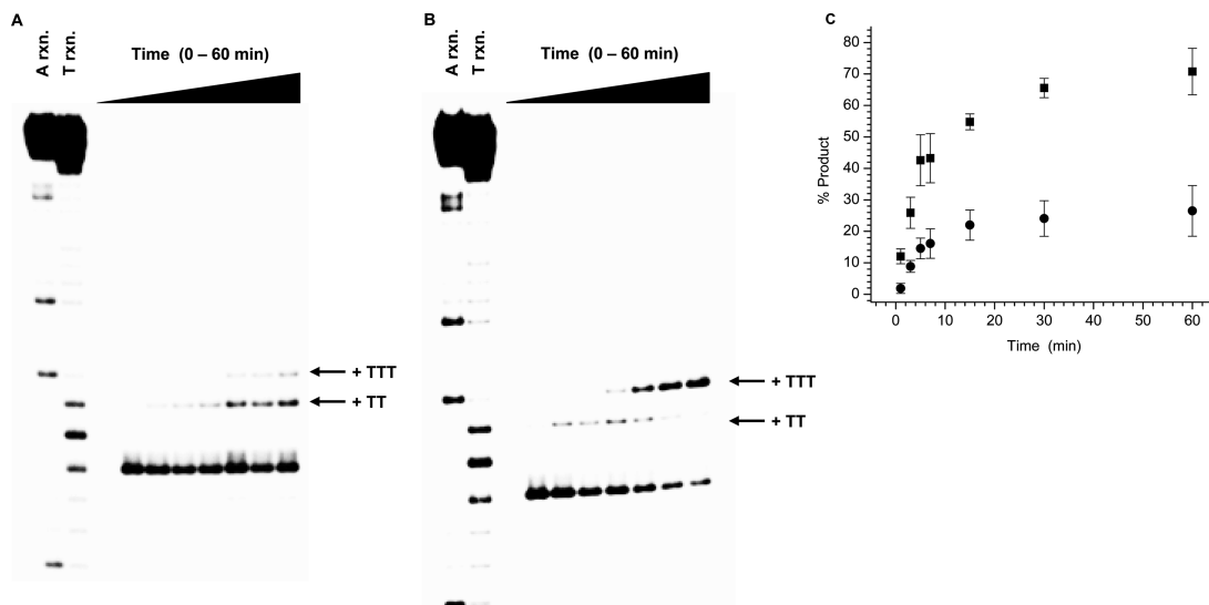
FIGURE 4: Strand displacement synthesis on 5'- 32 P-8 by Pol β (5 nM). (A) Extension as a function of time in the absence of FEN1. (B) Extension as a function of time in the presence of FEN1 (25 nM). (C) Total product formation as a function of time with FEN1 (square) and without FEN1 (circle). Sequencing reactions selective for T (T rxn) and A (A rxn).
