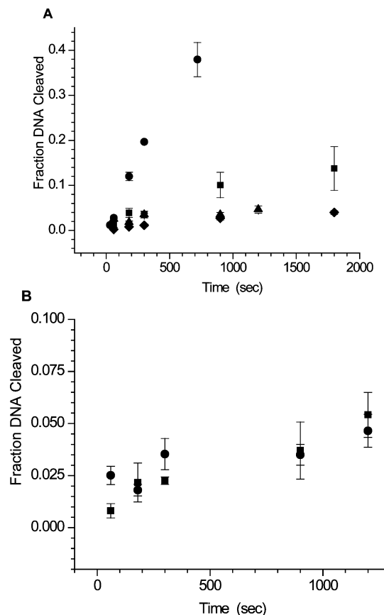
FIGURE 2: Excision of thymine glycol (Tg) by Nth as a function of time. (A) Tg ( 1 ), circle; LTg ( 3 ), triangle; -1 cluster ( 5 ), square; +1 cluster ( 6 ), diamond. (B) LTg ( 3 ), circle; FTg ( 4 ), square. Note: [Nth] = 0.25 nM when acting on 1 and 100 nM for reactions with 3–6 .
